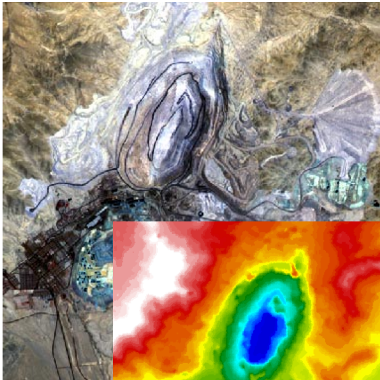
Full resolution examples of the DEM and VNIR imagery over the Chuquicamata Mine area.
